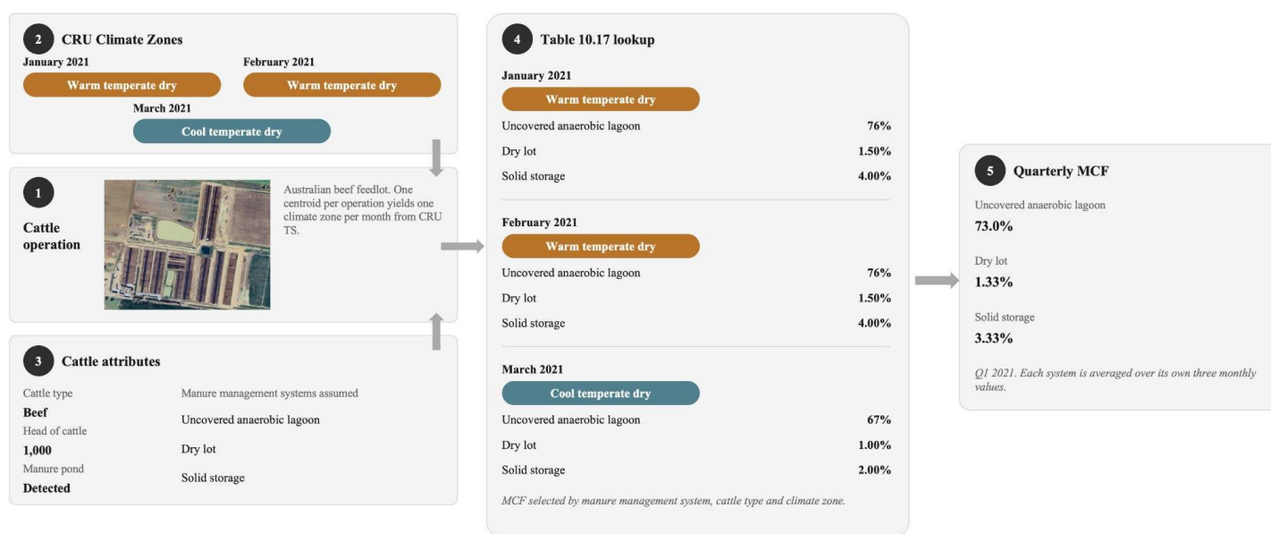
Figure 9 An example of deriving quarterly methane conversion factors (MCF) for a beef cattle operation, using an Australian feedlot in Q1 2021 as an example. (1) For an individual cattle operation identified by the AI detection models, the centroid per operation returned a (2) CRU TS climate zone for each month: warm temperate dry in January and February, cool temperate dry in March. (3) Cattle attributes assigned to the operation — beef, 1,000 head, manure pond detected — determine the multiple MMS assumed to be in use. (4) Cattle type, manure management system, and monthly climate zone together select an MCF from IPCC (2019) Table 10.17. (5) The three monthly values for each system were averaged to a quarterly MCF.
